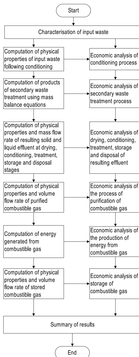
Figure 1. The program's computation procedure.
