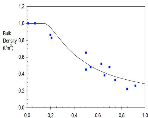
Figure 2. Variation of bulk density of sludge with bulk dryness.
