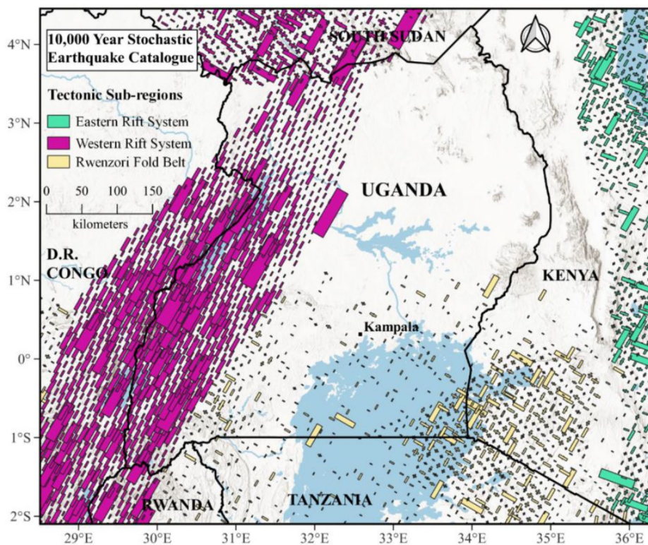
Fig. 10 Earthquake rupture geometries illustrating a 10,000-year subset of stochastic event catalogue striking each tectonic regime, following the major earthquakes ( M_w \geq 4.0 ) in Uganda
