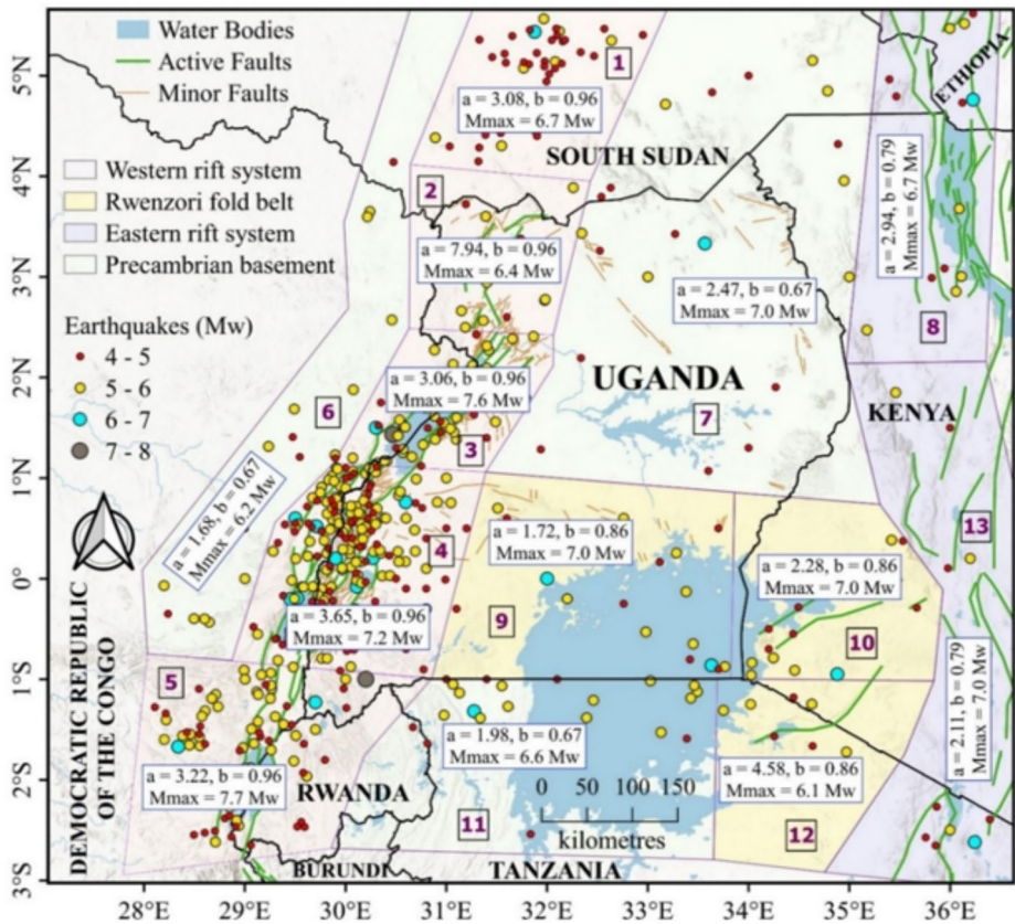
Fig. 5 Epicentres of M_w \geq 4.0 earthquakes which hit Uganda and its neighbouring countries between 1900 and 2022, major and minor active fault systems, area source zonation model and the calibrated seismicity parameters used to perform the stochastic event-based PSHA for Uganda
