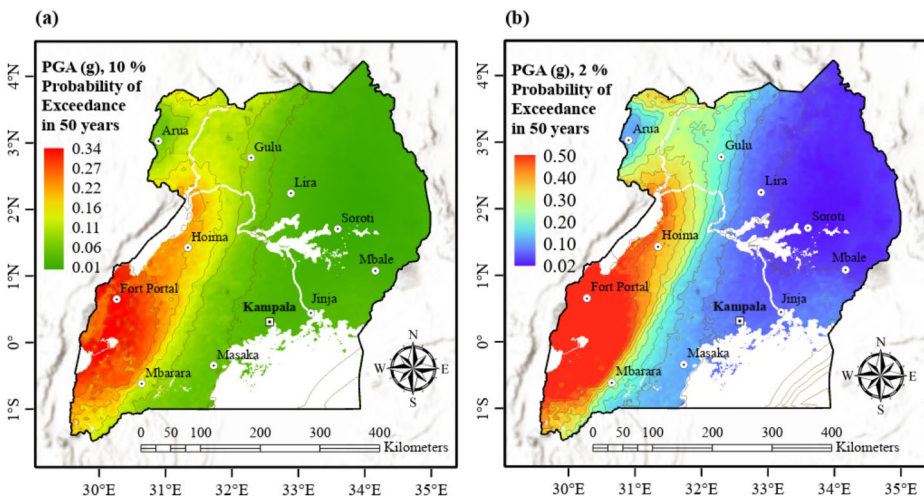
Fig. 12 Site-dependent seismic hazard maps of Uganda investigated over 50 years, in terms of PGA (g) and computed for: a 10% POE (475-year return period), and b 2% POE (2475-year return period). Contour lines are imposed on the maps at 0.05 g contour interval (Oleng et al. 2024b)
