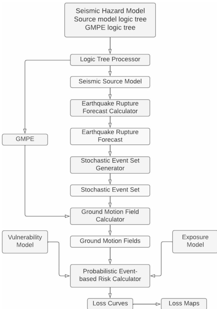
Fig. 4 Schematic diagram showing the chronological workflow of the probabilistic event-based risk and loss calculator embedded in the OpenQuake-engine
