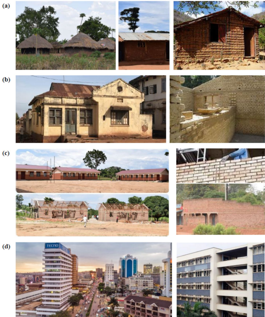
Fig. 6 Common building types constituting Uganda's building stock: a wattle-and-daub, b adobe with mud mortar, c fired bricks with cement mortar, and d modern-style buildings
